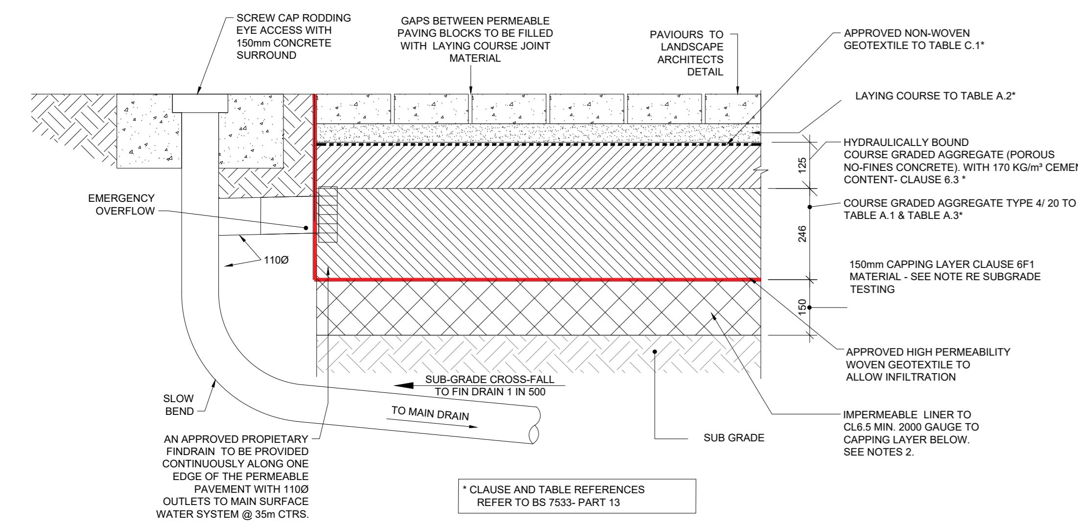
TYPICAL PERMEABLE PAVING DETAILS AND FIN DRAINAGE DETAILS SCALE @ A0: 1:10 SCALE @ A2: 1:20
