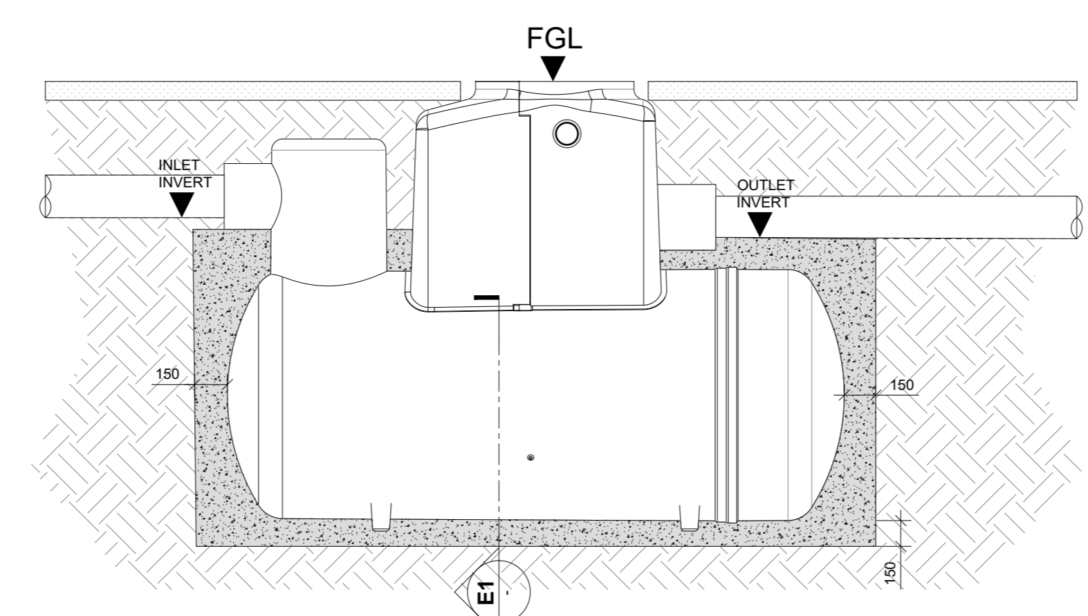
TYPICAL BYPASS PETROL INTERCEPTOR WITH CONCRETE SURROUND DETAILS SCALE @ A0: 1:25 SCALE @ A2: 1:50
