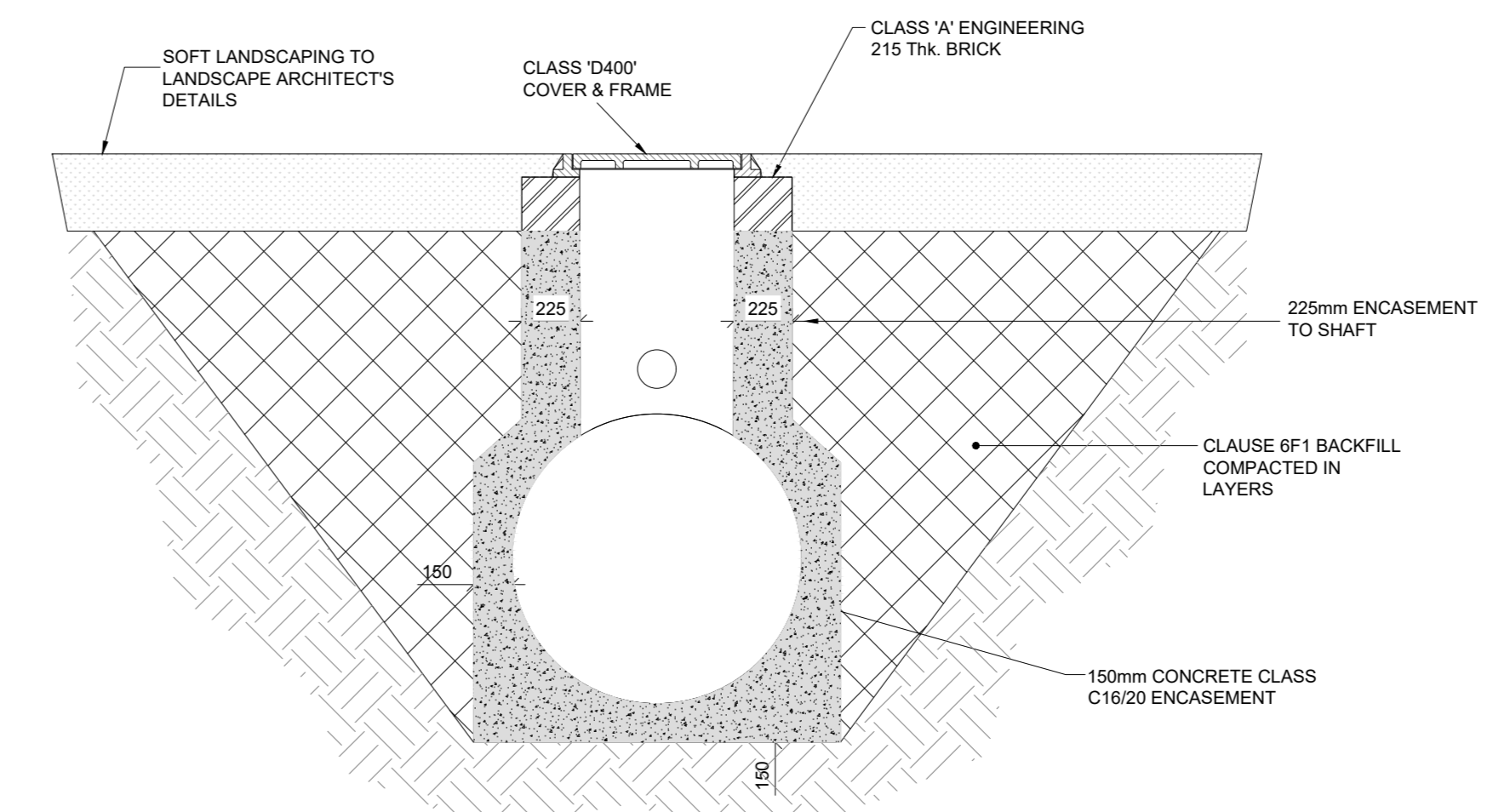
TYPICAL SECTION THROUGH PETROL INTERCEPTOR SHOWING CONCRETE SURROUND DETAIL SCALE @ A0: 1:25 SCALE @ A2: 1:50
